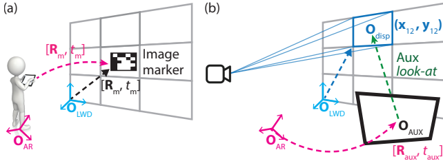
Figure 3: (a) Image marker used to align the aux AR coordinate system ( O_{AR} ) with the LWD physical space ( O_{LWD} ) at runtime. (b) This alignment allows AuxiScope to localize the aux relative to each LWD application instance.
