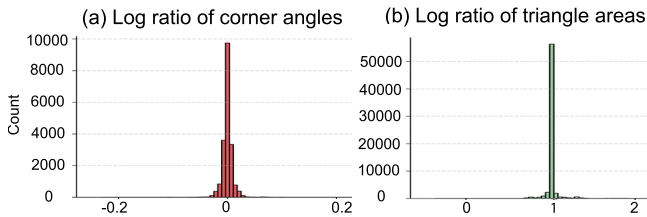
Figure 10: Histogram of log ratios for (a) conformal and (b) OT mapping, calculated for the capsule cubemap mesh projected on the Silo.
