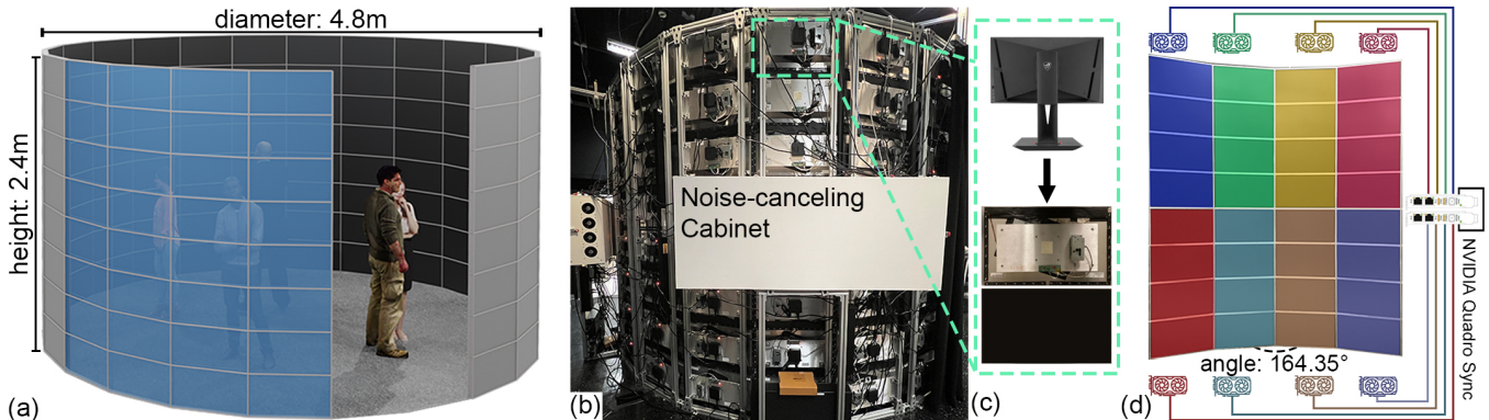
Figure 2: (a) 3D rendered diagram of the Silo model. (b) The back-side of one Silo node, showing our custom-designed aluminium mount frame and the noise canceling cabinet for the node server. (c) An inset showing our display customization from the manufacturer product, to reduce bezel size. (d) A diagram illustrating the GPU configuration in each node.
