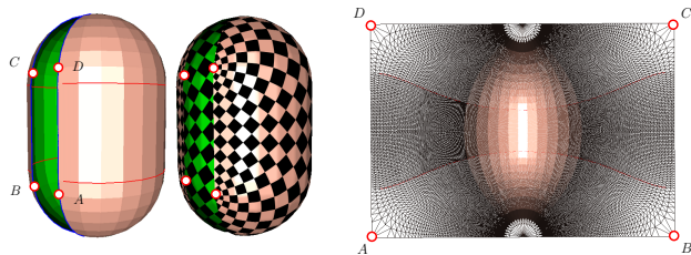
Figure 6: Conformal mapping preserves right angles.
