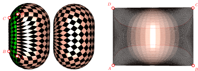
Figure 8: The composition of the conformal and the OT mapping is area-preserving. All checkers have the same size.
